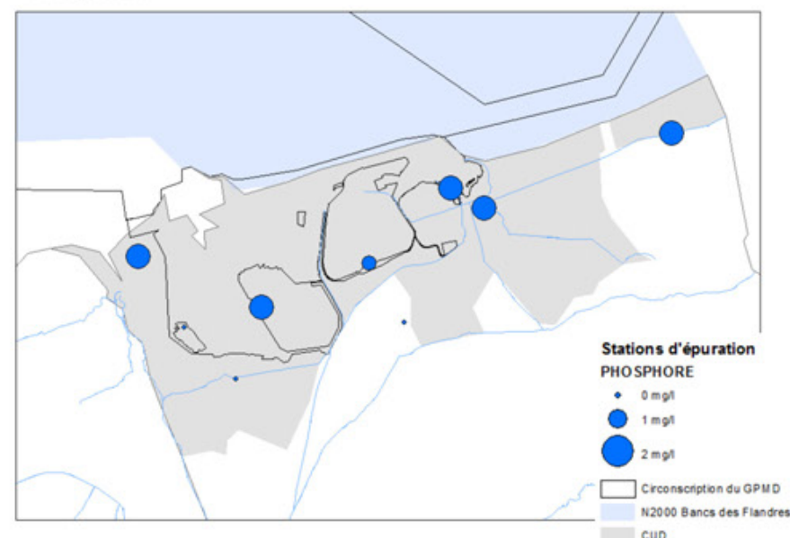
Phosphore
